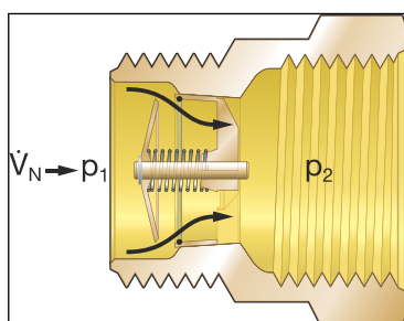
Fig. 3: Normal operation
