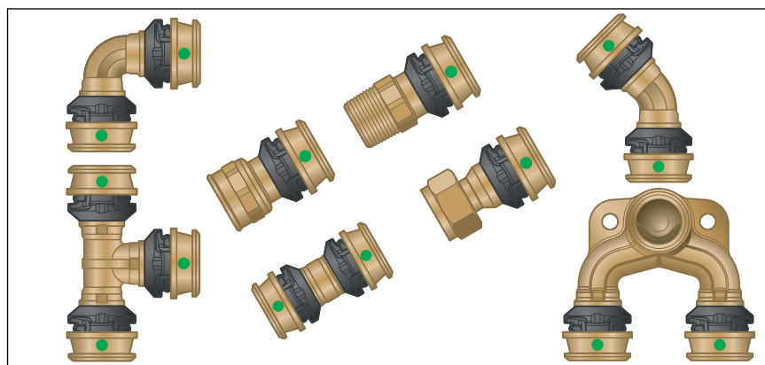
Fig. 1: Raxofix-presskoblinger
