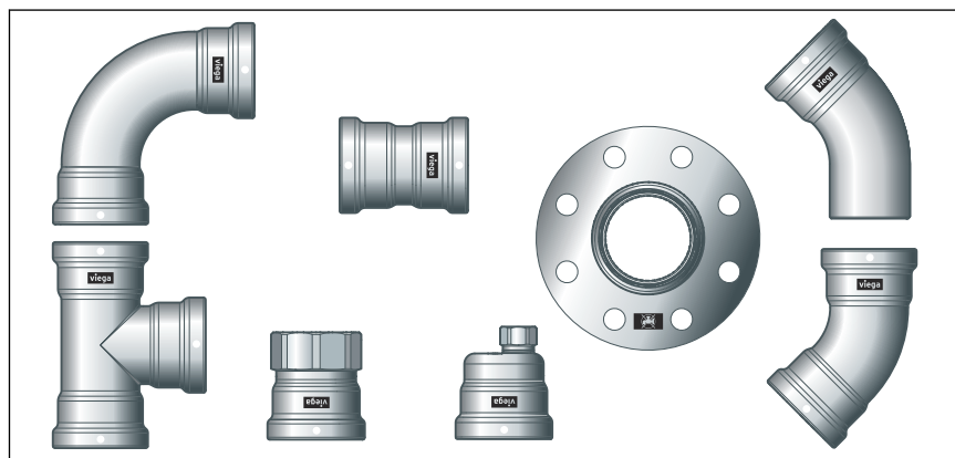
Fig. 2: Megapress S XL-presskoblinger
