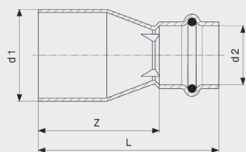
Seapress overgang - CuNiFe Modell 0315.1
