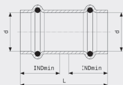
Seapress glidemuffe - CuNiFe Modell 0315.3
