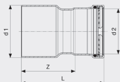
Seapress XL overgang - CuNiFe Modell 0315.1XL
