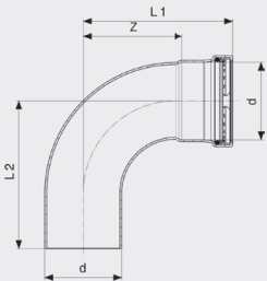
Seapress XL bend 90° - CuNiFe Modell 0316.1XL
