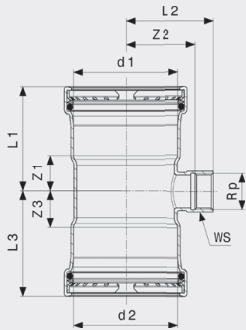
Seapress XL T-stykke - CuNiFe Modell 0317.2XL
