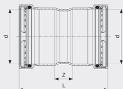
Seapress XL muffe - CuNiFe Modell 0315XL
