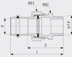
Seapress tippunion - CuNiFe Modell 0365.5
