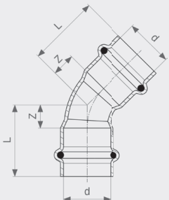
Seapress bend 45° - CuNiFe Modell 0326
