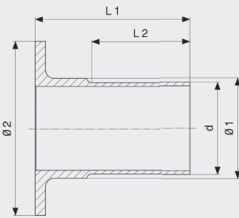
Seapress flens - CuNiFe Modell 0359.3
