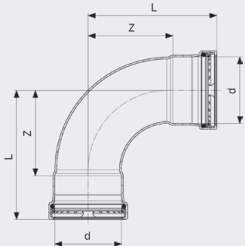
Seapress XL bend 90° - CuNiFe Modell 0316XL
