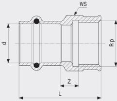
Seapress overgangsmuffe - CuNiFe Modell 0312
