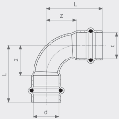
Seapress bend 90° - CuNiFe Modell 0316
