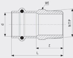
Seapress nippelmuffe - CuNiFe Modell 0311.5
