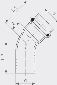
Seapress bend 45° - CuNiFe Modell 0326.1
