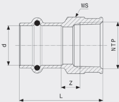
Seapress overgangsmuffe - CuNiFe Modell 0312.5
