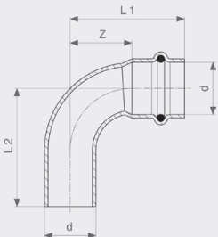
Seapress bend 90° - CuNiFe Modell 0316.1
