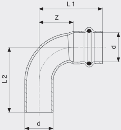
Profipress S bend 90° - kobber Modell 4516.1
