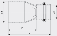
Profipress S overgang - kobber Modell 4515.1
