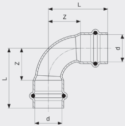
Profipress S bend 90° - kobber Modell 4516
