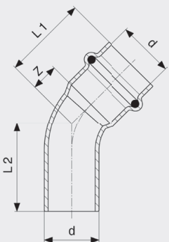
Profipress S bend 45° - kobber Modell 4526.1
