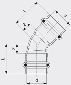
Profipress S bend 45° - kobber Modell 4526
