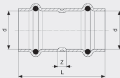
Profipress S muffe - kobber Modell 4515
