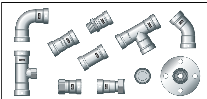
Afb. 2: Megapress S-persfittings
