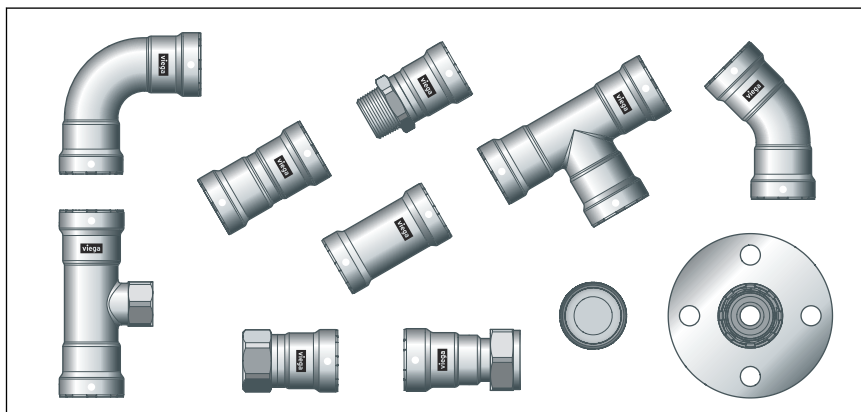
Afb. 2: Megapress S-persfittingen
