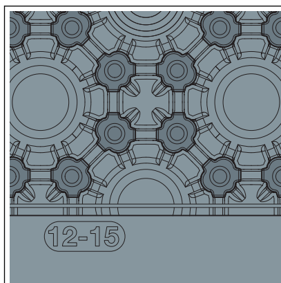
Fig. 1: Detailed view of dimple geometry 12/15
