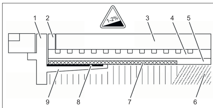
Fig. 2: Construction diagram of the bonded seal - min. screed incline 1–2 %
