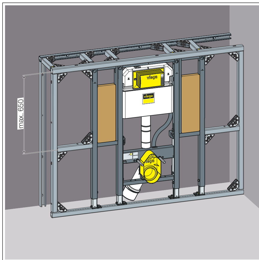
Fig. 5: Montage sans obstacles, variante 1
