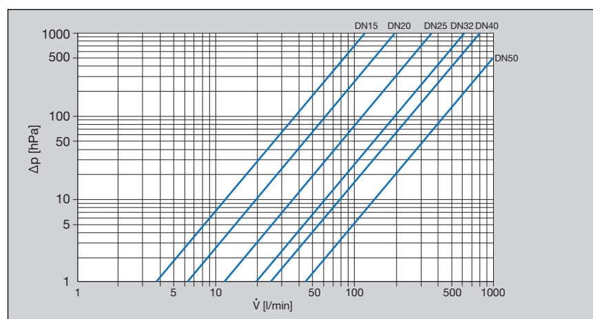
Fig. 1: Performance diagram slanted seat valve press/threaded connection
