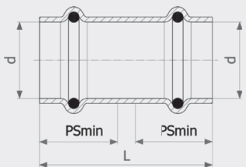
Seapress liukumuhvi - CuNiFe malli 0315.3
