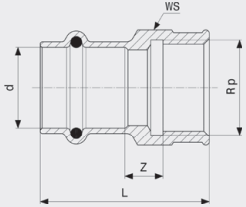
Seapress nippa - CuNiFe malli 0312
