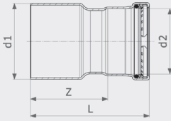
Seapress XL supistus - CuNiFe malli 0315.1XL
