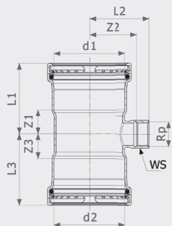
Seapress XL T-yhde - CuNiFe malli 0317.2XL
