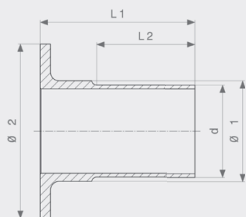
Seapress XL kaulus - CuNiFe malli 0359.3XL
