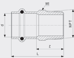
Seapress nippa - CuNiFe malli 0311.5
