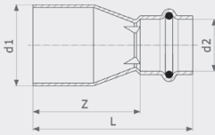
Seapress supistus - CuNiFe malli 0315.1
