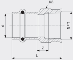
Seapress nippa - CuNiFe malli 0312.5
