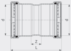
Seapress XL muhvi - CuNiFe malli 0315XL
