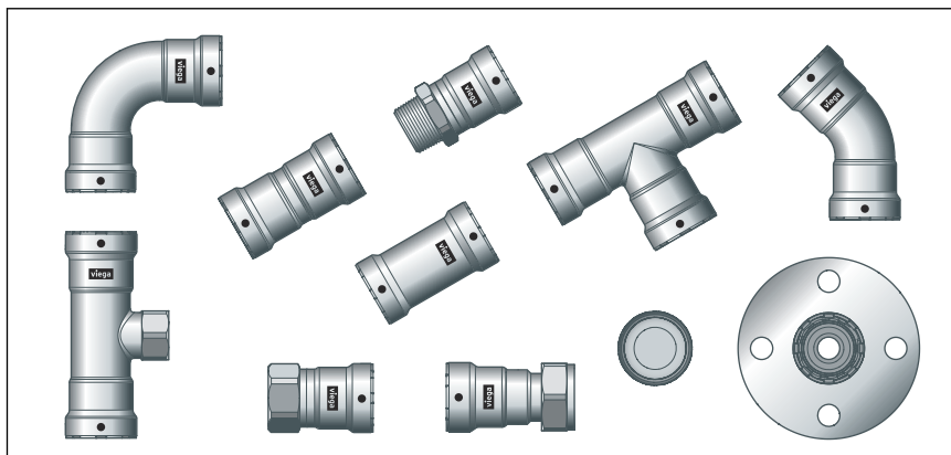
Abb. 2: Megapress-Pressverbinder
