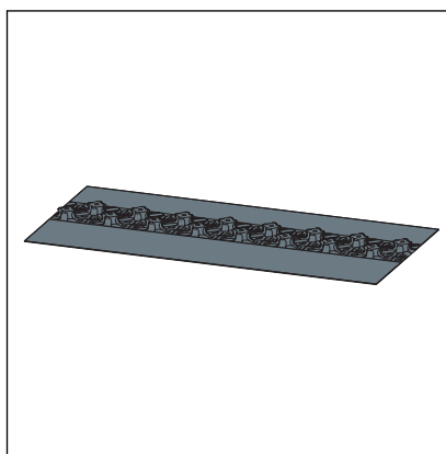
Fig. 2: Example illustration - dimple geometry may deviate Smart Fonterra Base-door element, for on-site insulation.
